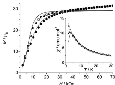
Figure 2. Field dependence of the molar magnetization measured on a pellet of polycrystalline powder of Dy 6 at T = 1.8\text{ K} (●) and T = 4.0\text{ K} (□). Inset: temperature dependence of the magnetic susceptibility on a polycrystalline powder at H = 1\text{ kOe} (▲) and H = 10\text{ kOe} (○). Lines correspond to the calculated values (see text) obtained from the simultaneous simulation of single-crystal data.
